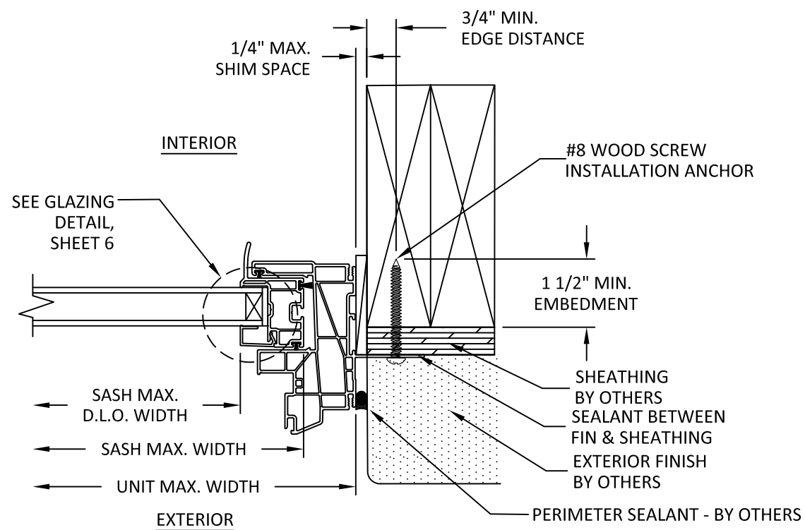
D 3 HORIZONTAL SECTION NAIL FIN INSTALLATION WOOD BUCK
