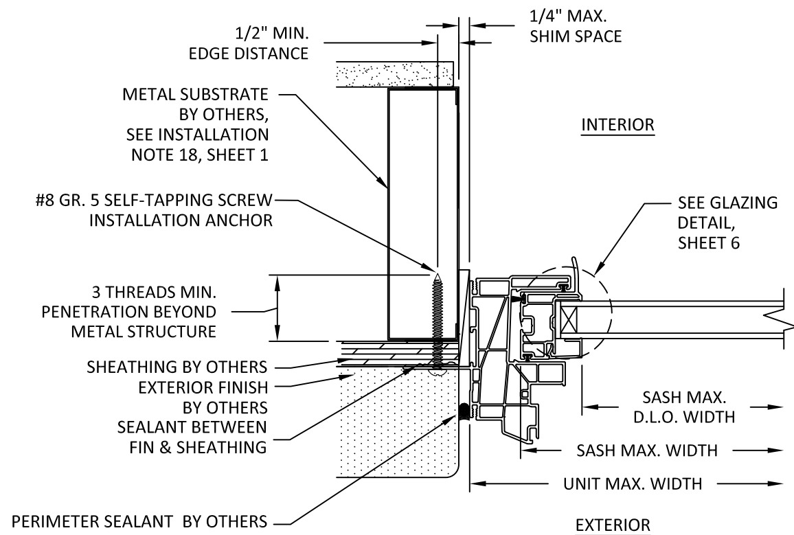
B 3 HORIZONTAL SECTION NAIL FIN INSTALLATION METAL STUD
