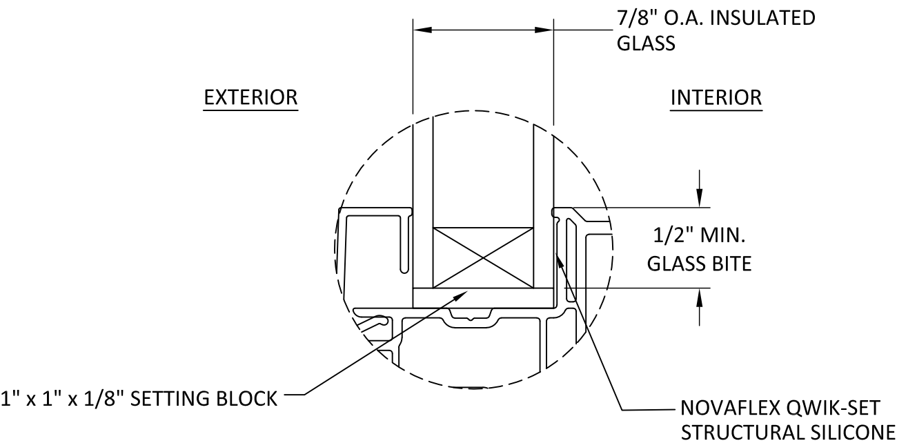
GLAZING DETAIL
