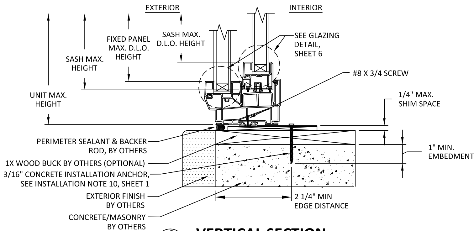
C 5 VERTICAL SECTION CLIP INSTALLATION CONCRETE/CMU
