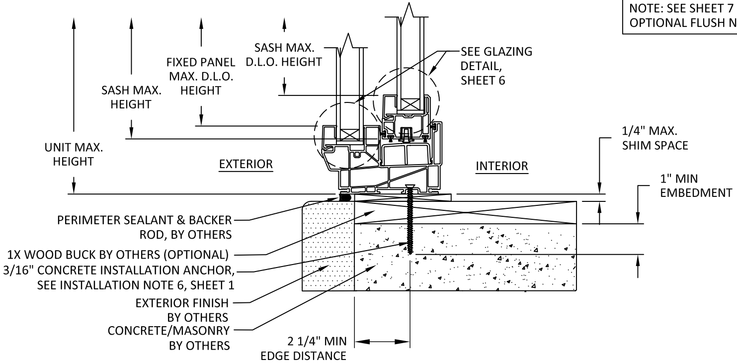
C 4 VERTICAL SECTION THROUGH FRAME INSTALLATION CONCRETE/CMU
