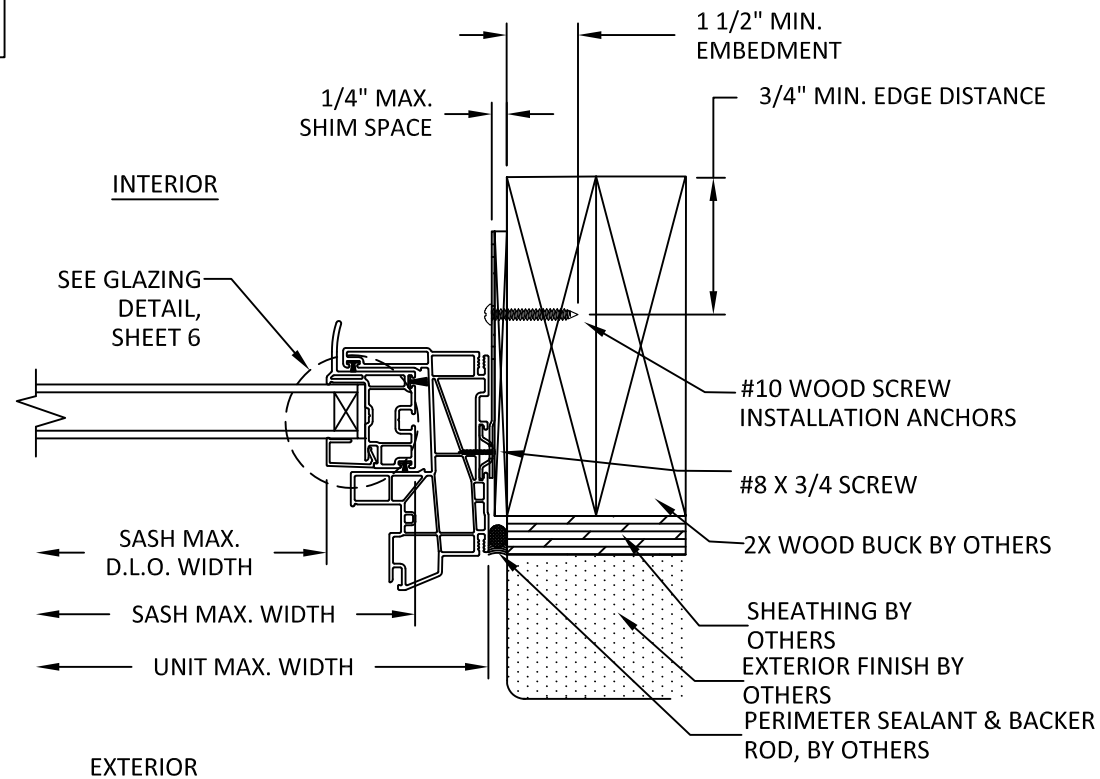
D 5 HORIZONTAL SECTION CLIP INSTALLATION WOOD BUCK
