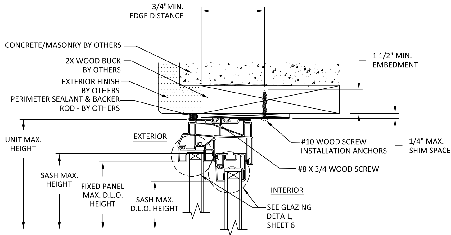
A 5 VERTICAL SECTION CLIP INSTALLATION WOOD BUCK
