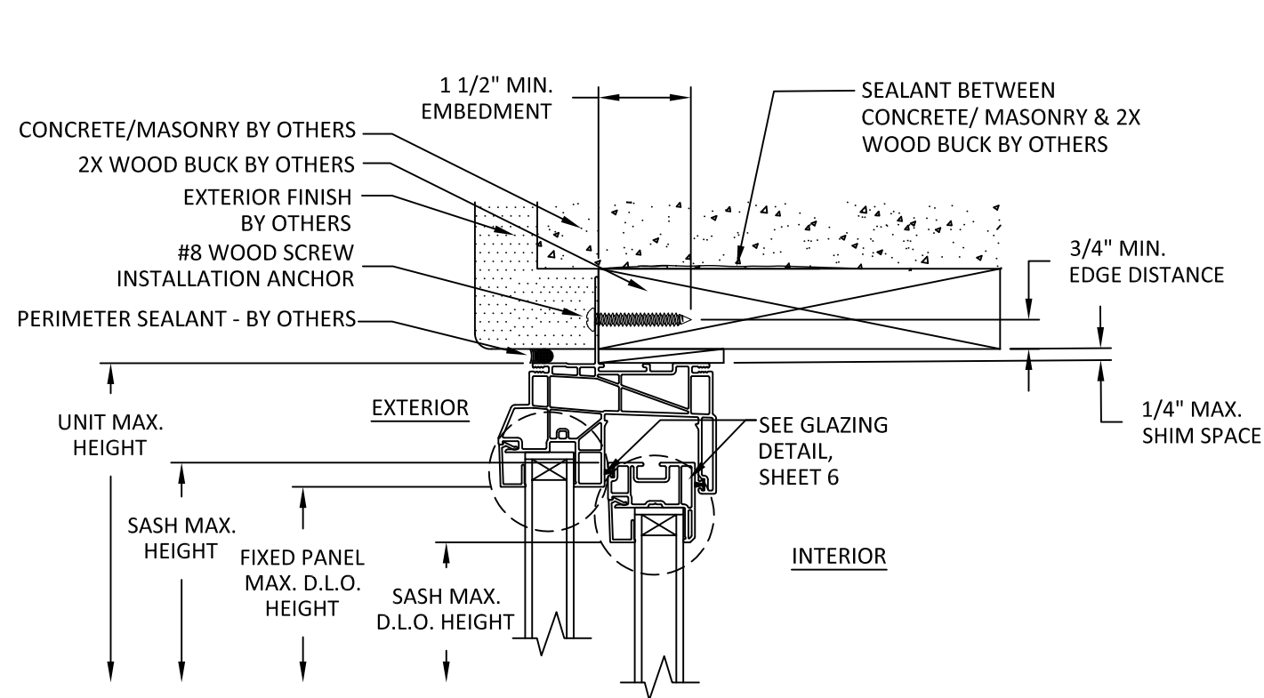
A 3 VERTICAL SECTION NAIL FIN INSTALLATION WOOD BUCK
