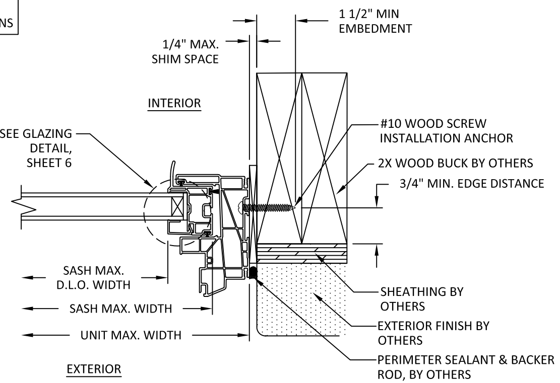
D 4 HORIZONTAL SECTION THROUGH FRAME INSTALLATION WOOD BUCK
