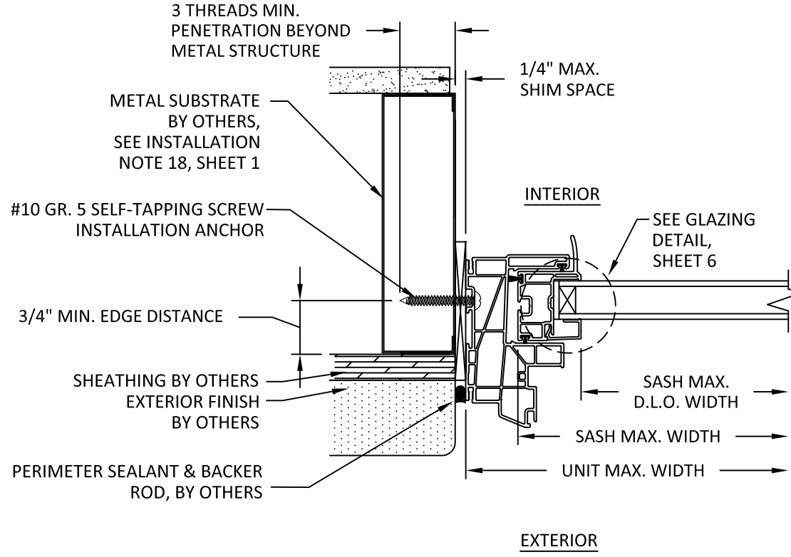
B 4 HORIZONTAL SECTION THROUGH FRAME INSTALLATION METAL STUD
