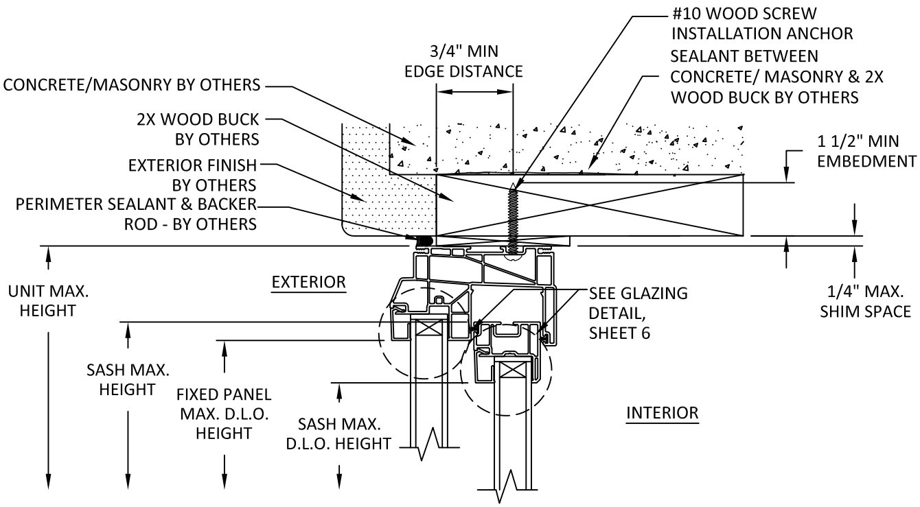
A 4 VERTICAL SECTION THROUGH FRAME INSTALLATION WOOD BUCK
