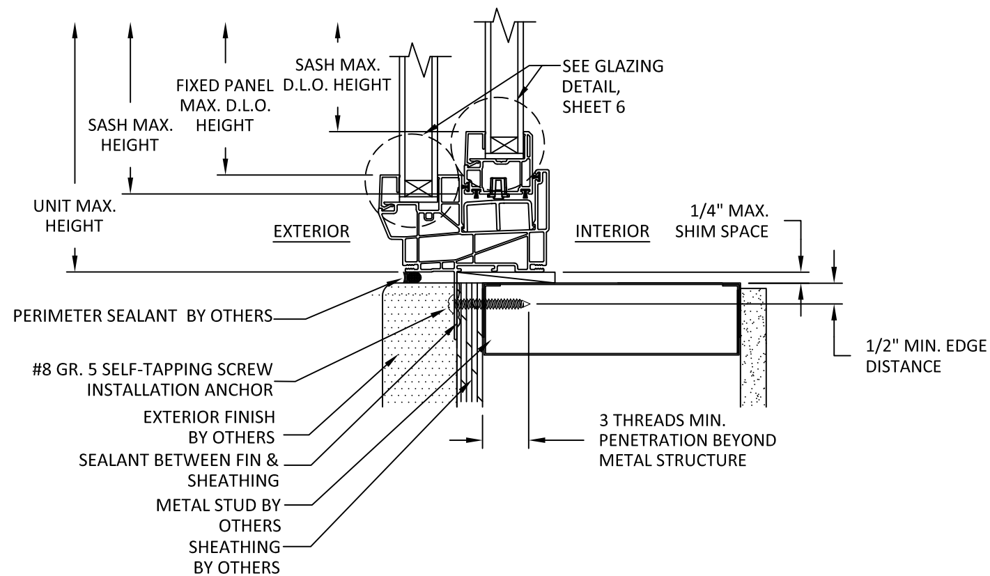
C 3 VERTICAL SECTION NAIL FIN INSTALLATION METAL STUD
